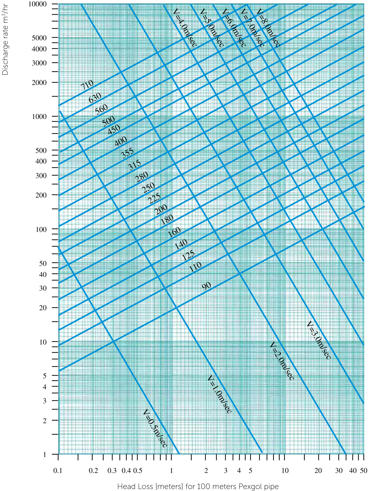
Chart 18.1: Class 6 (SDR 26)
