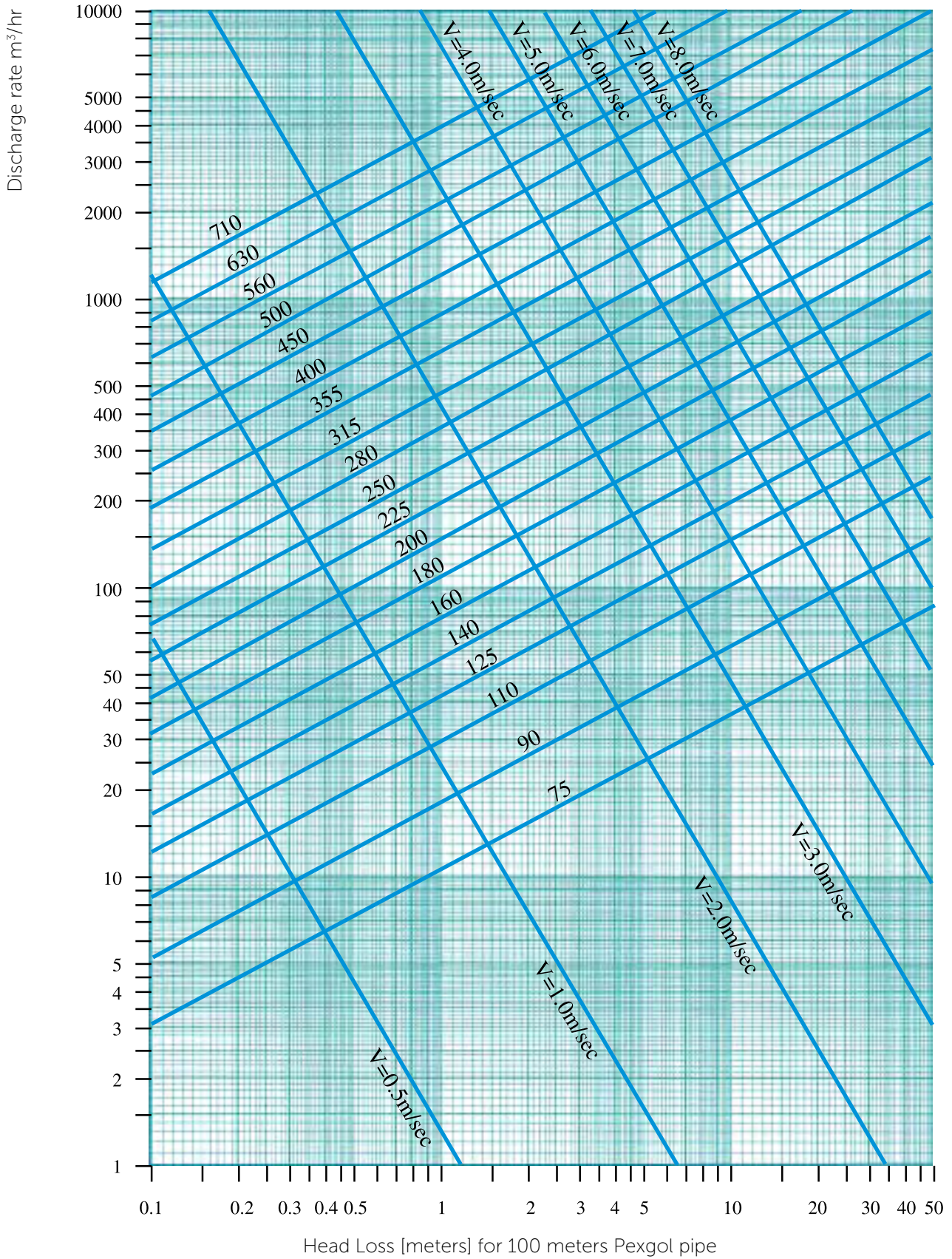
Chart 19.1: Class 8 (SDR 21)
