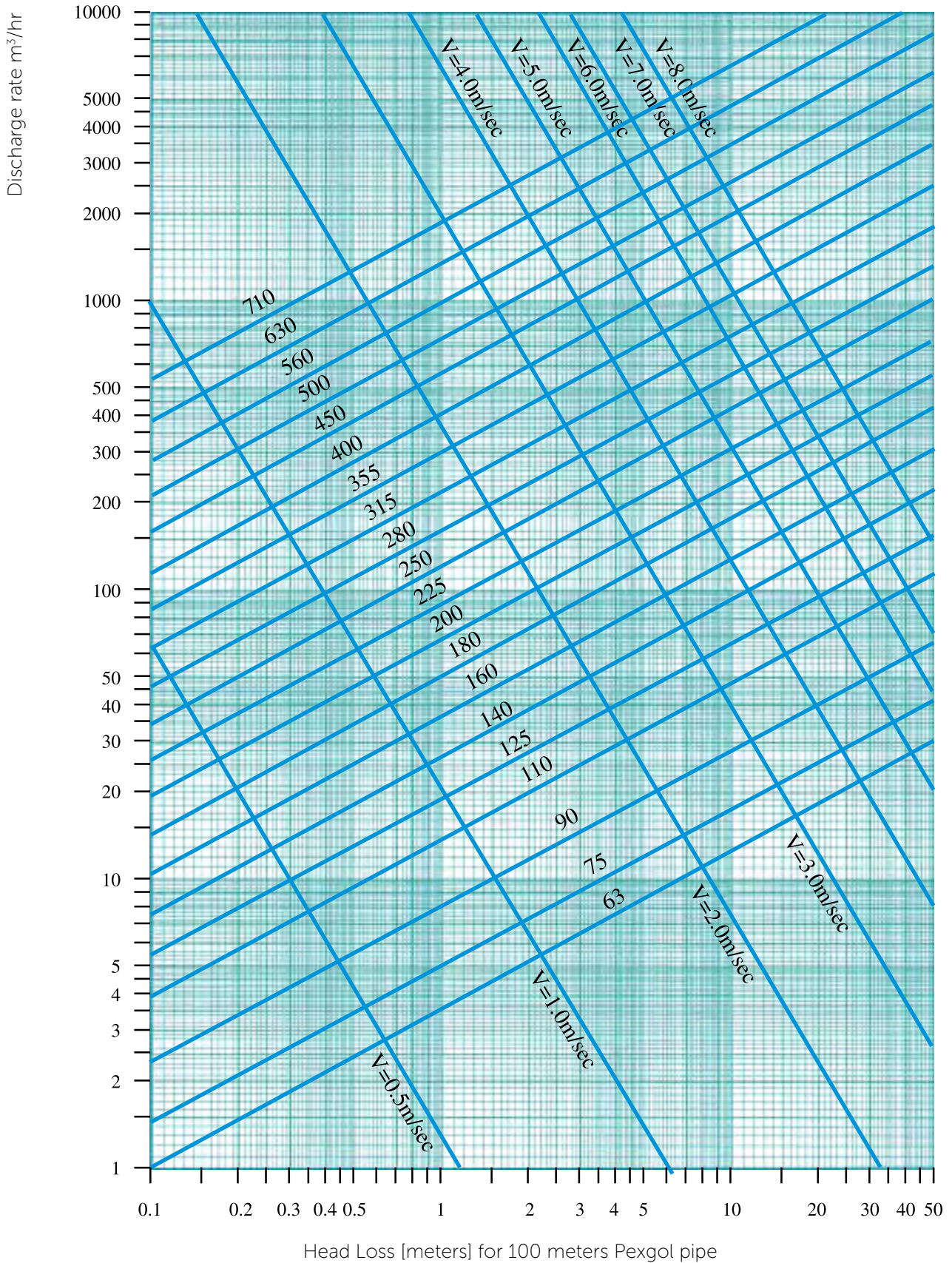
Chart 25.1: Class 30 (SDR 6)
