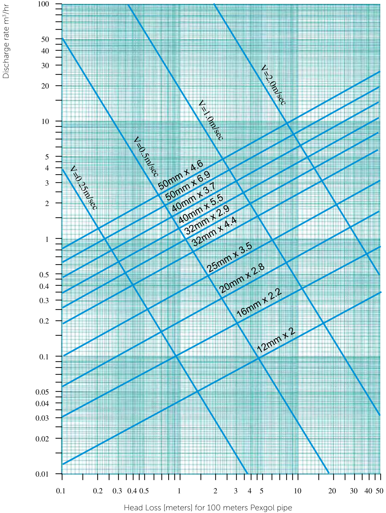
Chart 26.1: Class 24 (SDR 7.4) and Class 15 (SDR 11)
