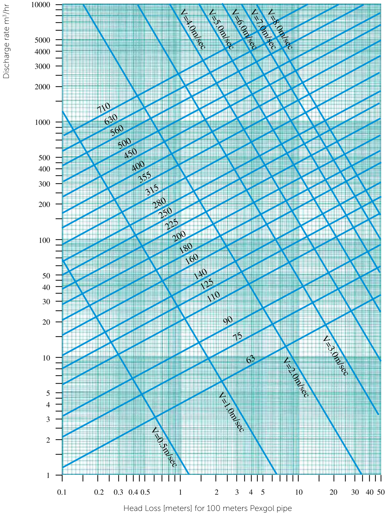
Chart 23.1: Class 19 (SDR 9)
