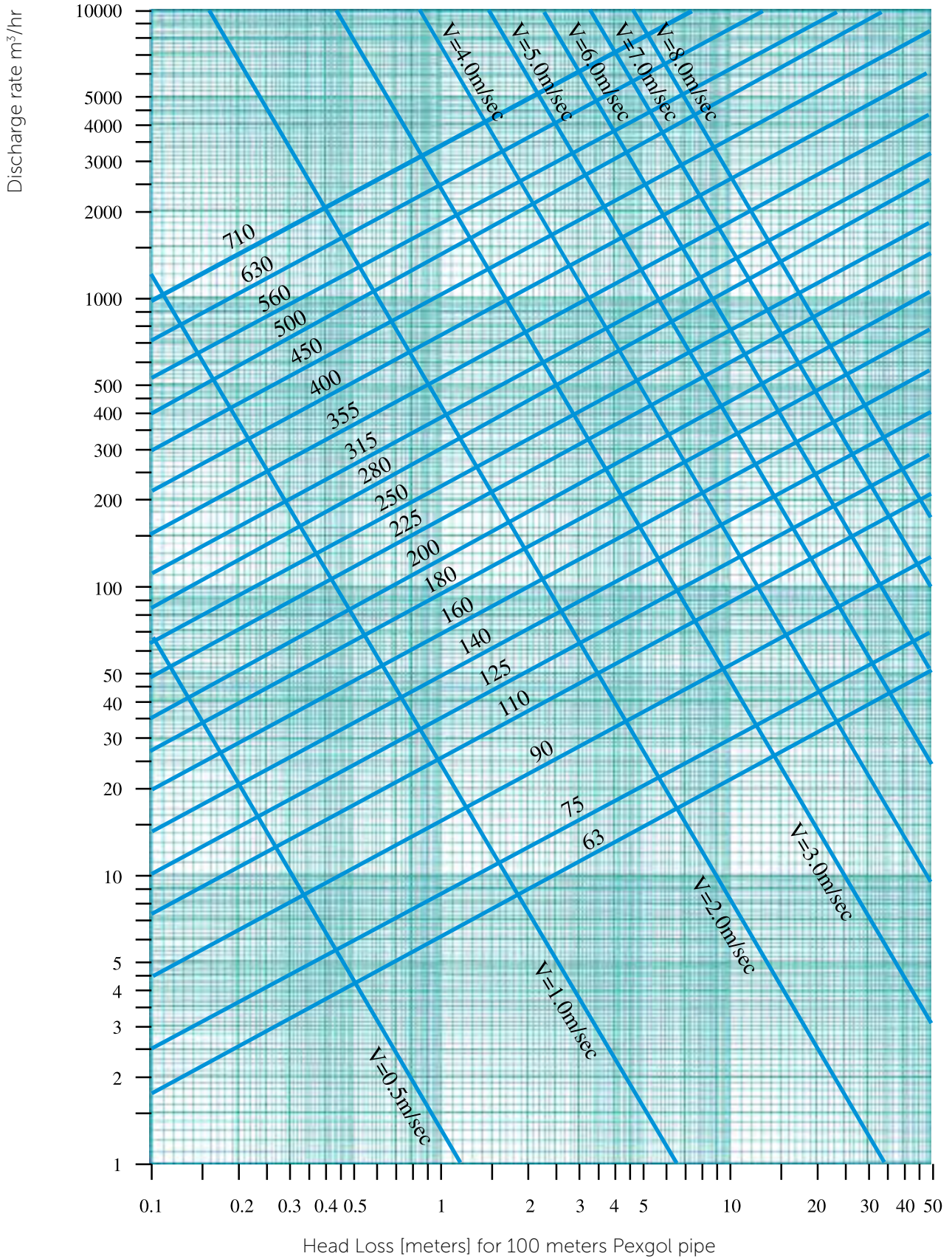
Chart 21.1: Class 12 (SDR 13.6)
