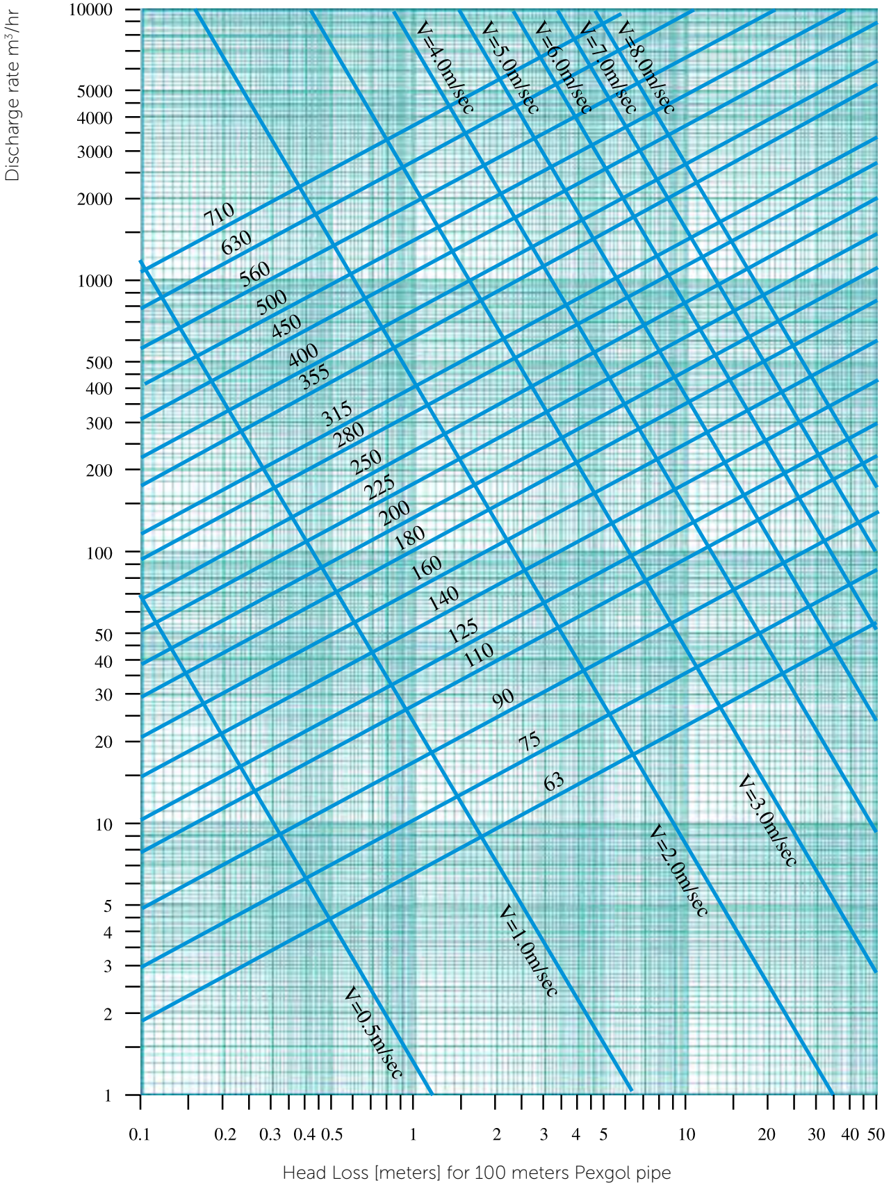
Chart 20.1: Class 10 (SDR 16.2)
