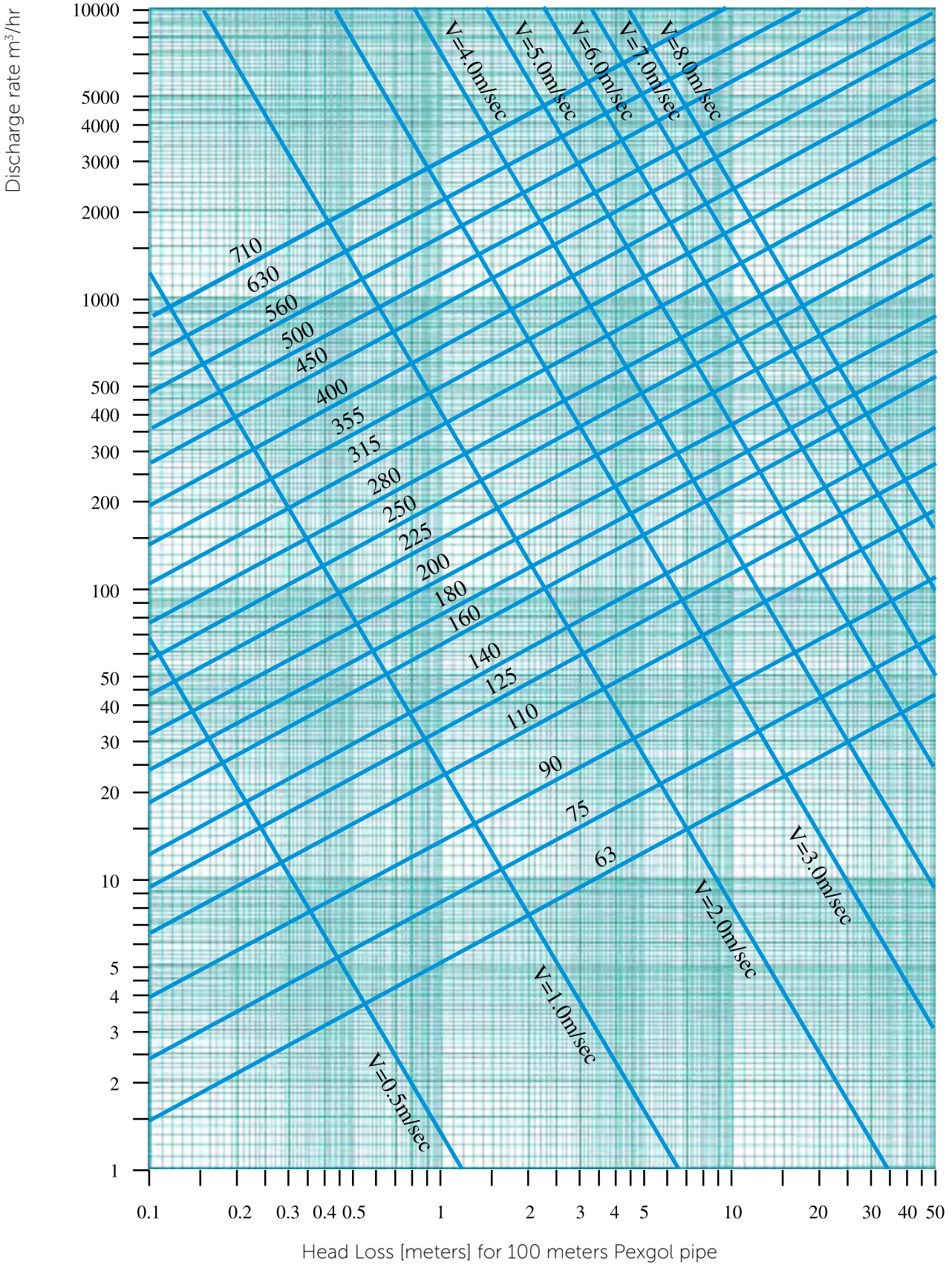
Chart 22.1: Class 15 (SDR 11)
