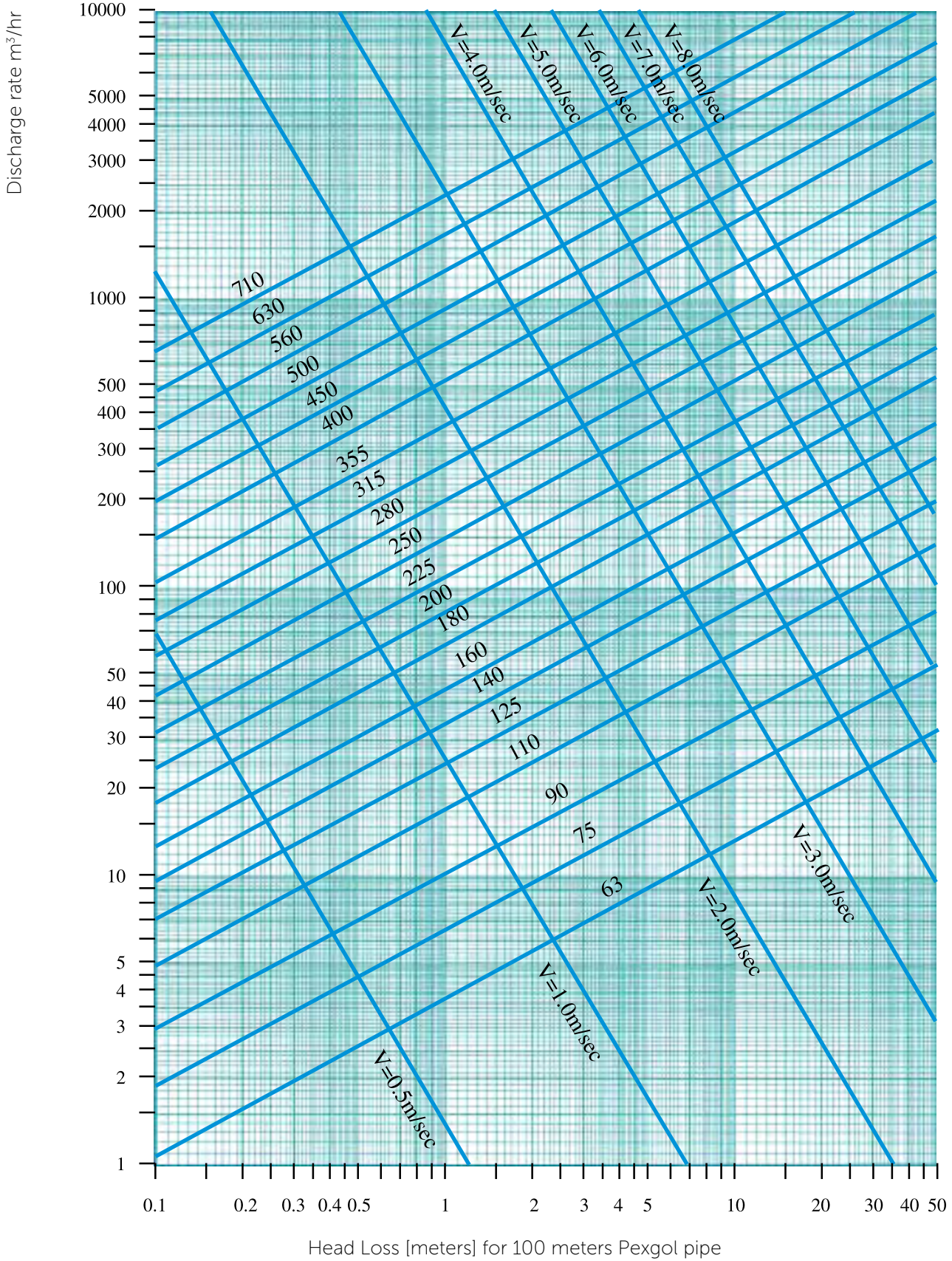
Chart 24.1: Class 24 (SDR 7.4)
